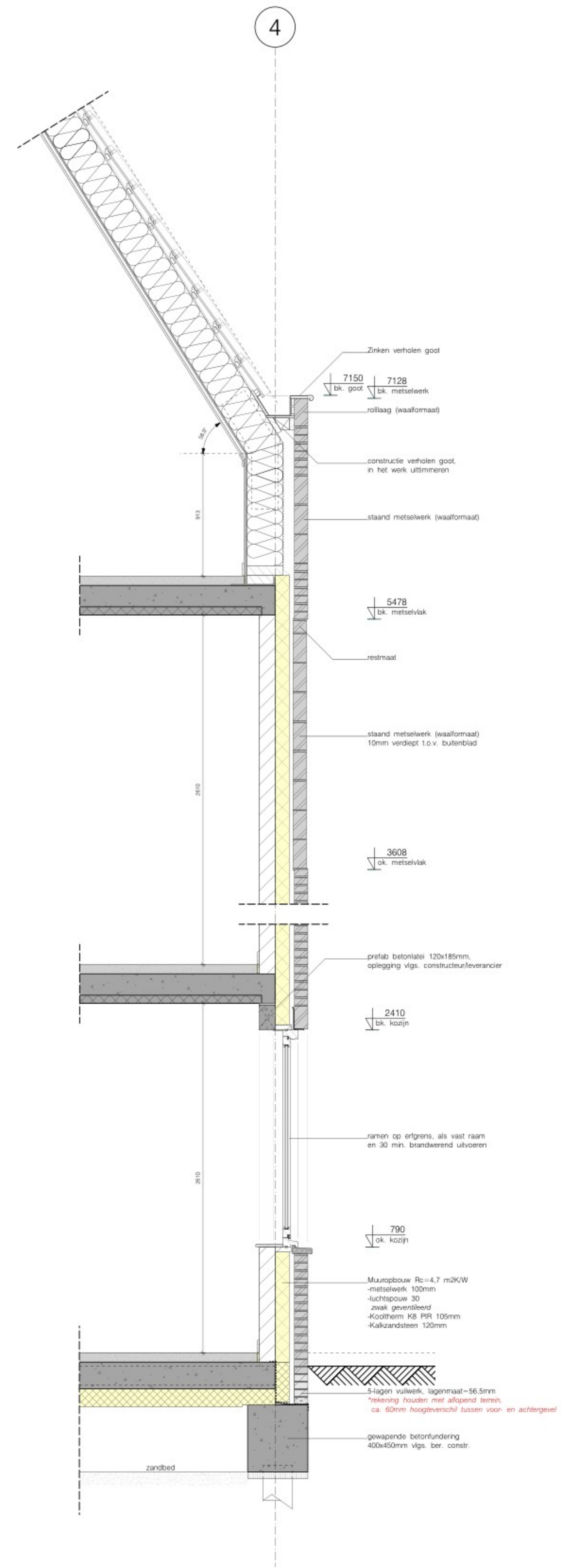
PRINCIPE DETAIL 11 zigevel woning 43
