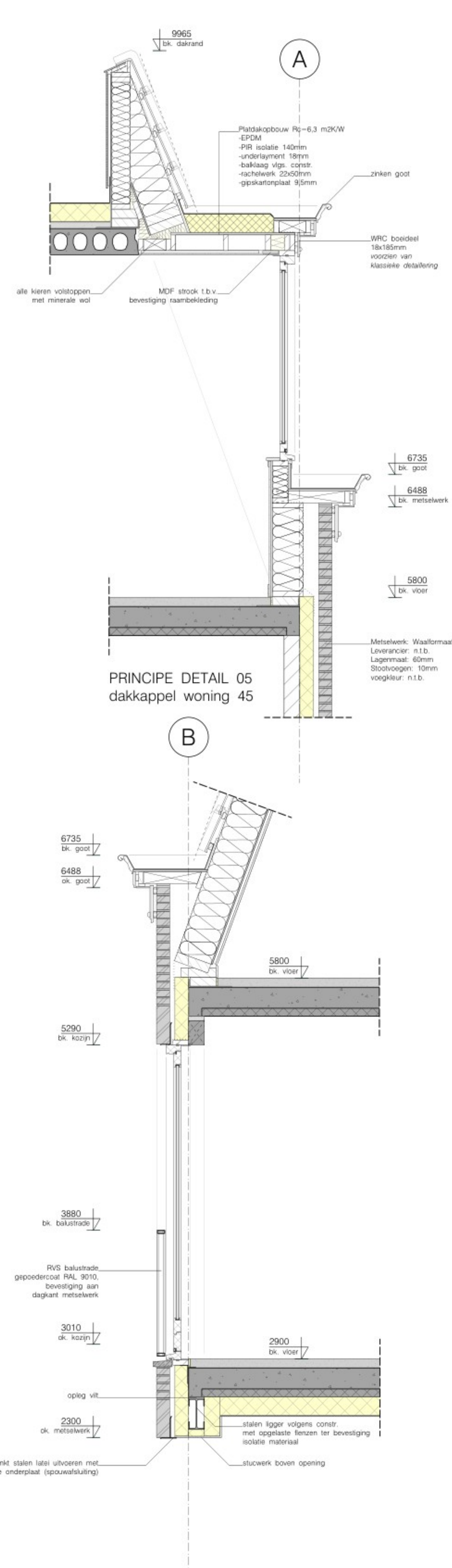
PRINCIPE DETAIL 05 dakkappel woning 45
